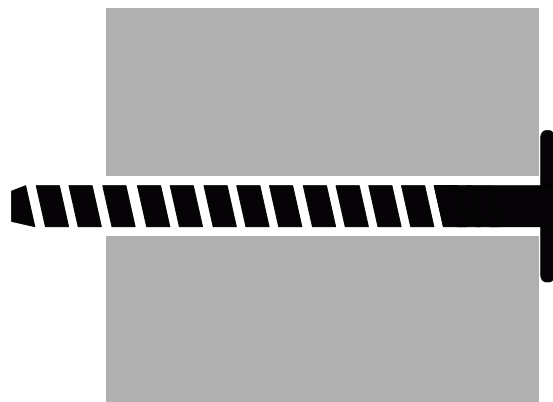
2 1/4"(56mm) PANEL 70mm CONNECTOR BOLT TO FASTEN RODS
